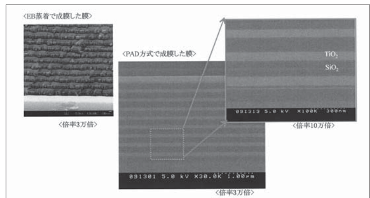
図11 \text{TiO}_2/\text{SiO}_2 多層膜断面の電子顕微鏡観察 Fig.11 Electron microscope observation of the multiple layers ( \text{TiO}_2/\text{SiO}_2 ) film sections
