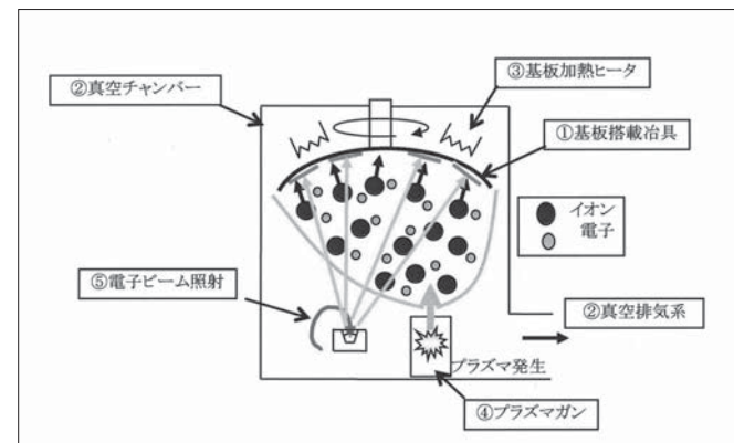
図2 PAD方式の模式図 Fig.2 Schematic drawing of PAD
