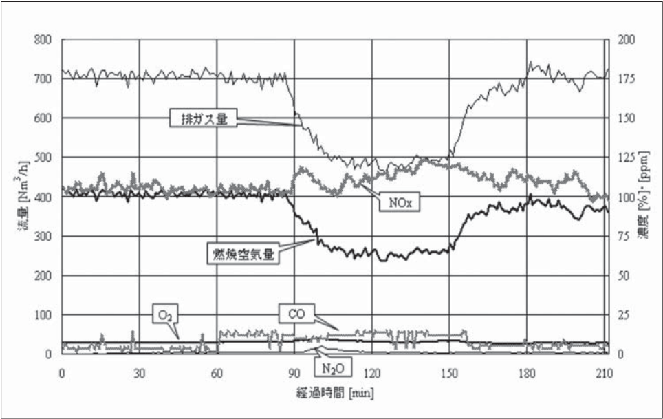
図16 汚泥供給量変化による排ガス性状変化 Fig.16 NOx, N 2 O and CO of pilot plant during low feeding
