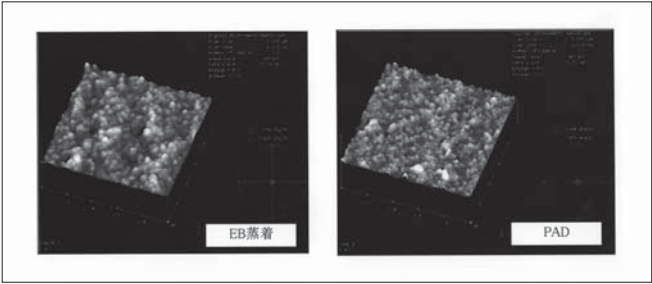
図16 膜表面の原子間力顕微鏡での観察結果 Fig.16 Result of observation with atomic force microscope on the surface of multiple layers (TiO 2 /SiO 2 ) film
