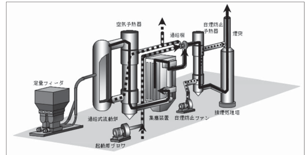
図1 開発システム Fig.1 Flow chart of Fluidized Bed Incinerator with the turbocharger
