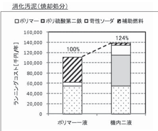
図20 ランニングコストの比較(処理場規模150,000m 3 /日、焼却処分) Fig.20 Comparison of running cost (Plant scale 150,000m 3 /day, incineration disposal on same site) (Polymer flocculant conditioning vs two-flocculant conditioning)
