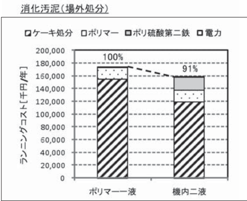
図19 ランニングコストの比較(処理場規模50,000m 3 /日、場外処分) Fig.19 Comparison of running cost (Plant scale 50,000m 3 /day, outside disposal) (Polymer flocculant conditioning vs two-flocculant conditioning)
