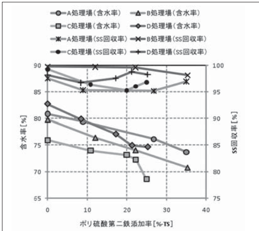
図16 機内二液調質法実験結果(消化汚泥) Fig.16 Test results of two-flocculant conditioning method (anaerobic digestion sludge)
