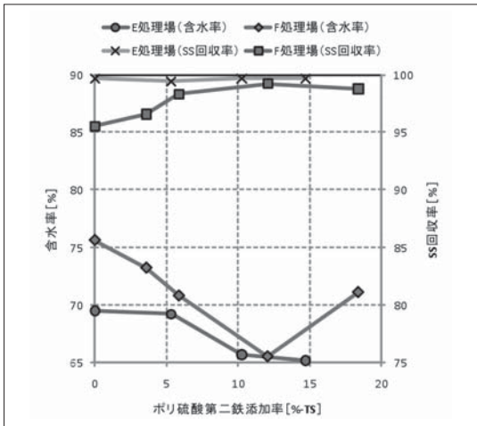
図17 機内二液調質法実験結果(混合生汚泥) Fig.17 Test results of two-flocculant conditioning method (mixed raw sludge)
