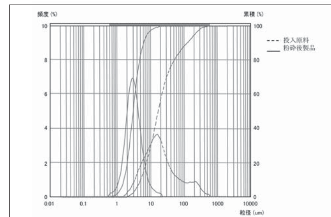
図2 酸化チタン系材料の粉砕前後の粒度分布 Fig.2 Particle size distribution before and after pulverized TiO2-based material
