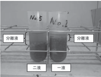
図10 一液と二液の脱水性の差異 Fig.10 The difference of dewatering performance between using polymer flocculant and two-flocculant conditioning by spin tube test
