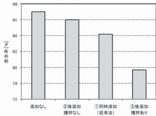
図9 ビーカー試験による二液法の比較 Fig.9 The results of spin tube test using two-flocculant conditioning method
