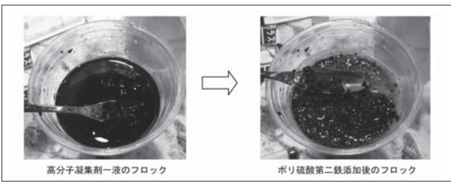
図8 一液と二液のフロック形成の違い Fig.8 The difference of floc formation between using polymer flocculant and adding poly-ferric sulfate solution
