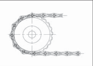
図6 浮上型チェーン巻き付き状態 Fig.6 The chain volubile state of the floating type
