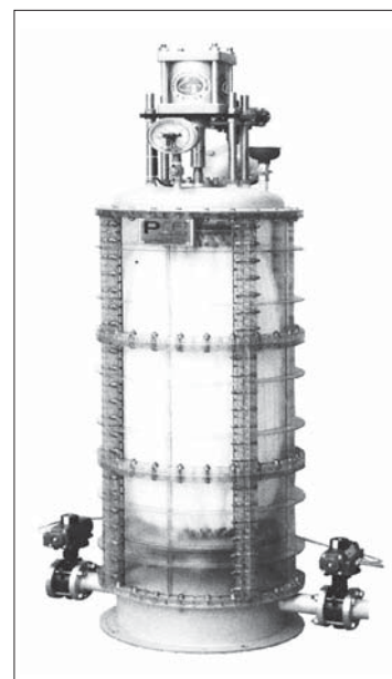
図2 PCF Filter Fig.2 Photo of PCF Filter
