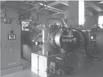
図13 岐阜市雄総水源 実績写真 (最大水量: 55,296m 3 /日) Fig.13 Operational UV equipment at Gifu Pref. (Maximum flow rate: 55,296m 3 /day)
