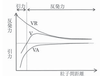
図4 汚泥粒子に働く力と距離の関係 3) Fig.4 The Relationship between the force acting on sludge particle and distance from sludge particle
