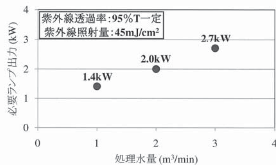
図9 処理水量と必要ランプ出力の関係 Fig.9 Relation between flow rate and requisite lamp output
