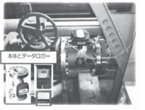
図14 自動水分計の設置状況 Fig.14 State of installation of automatic water content meter
