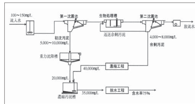
図1 下水処理過程における固形物濃度(例) Fig.1 Dry substance of sludge in sewage sludge treatment process
