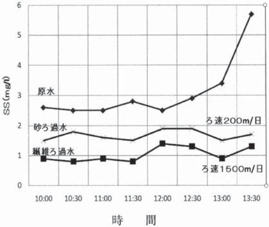
図4 浮遊物質の比較 Fig.4 Comparison of SS concentration in raw water and filtrate
