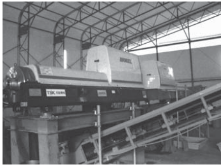
図6 仮設脱水機運転の状況 Fig.6 Operational condition of the temporary dewatering machine
