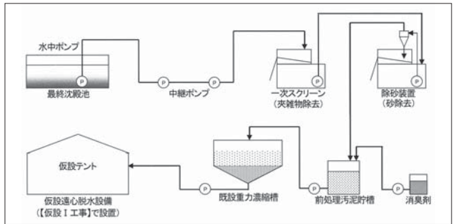
図7 最終沈殿池堆積汚泥の浚渫処理フロー Fig.7 Dredging operation flow for mud at final sedimentation tank
