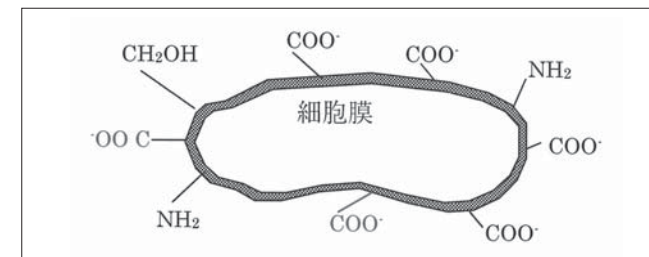
図2 汚泥粒子の表面荷電状態 Fig.2 The condition on surface of sludge particle
