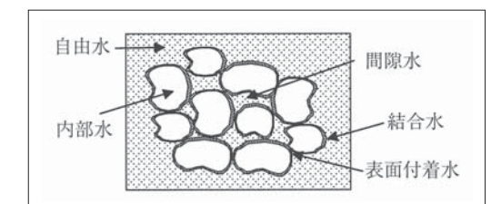
図5 汚泥中の水分の存在状態 4) Fig.5 Existing condition of water content in sludge
