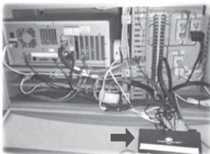
図3 KVMスイッチ(汚泥棟監視室) Fig.3 KVM switch in the monitoring room
