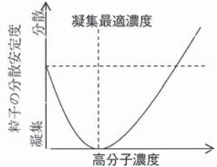
図9 粒子の分散安定度と高分子濃度の関係 5) Fig.9 The relationship between stability of dispersion and concentration of polymer flocculant
