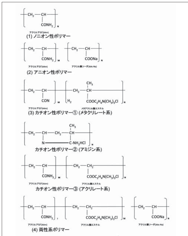
Fig.12 Molecular structure of typical polymer flocculant
